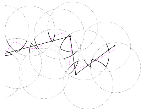
Figure 6. The path computed by OCCAMTRACK has 3 line segments. The sequence of arcs delineating the regions of band B are shown in thick lines.
